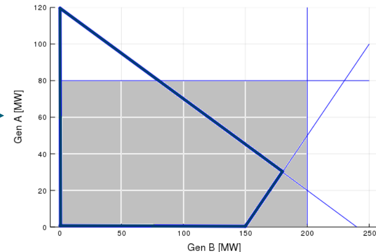
Transmission switching
