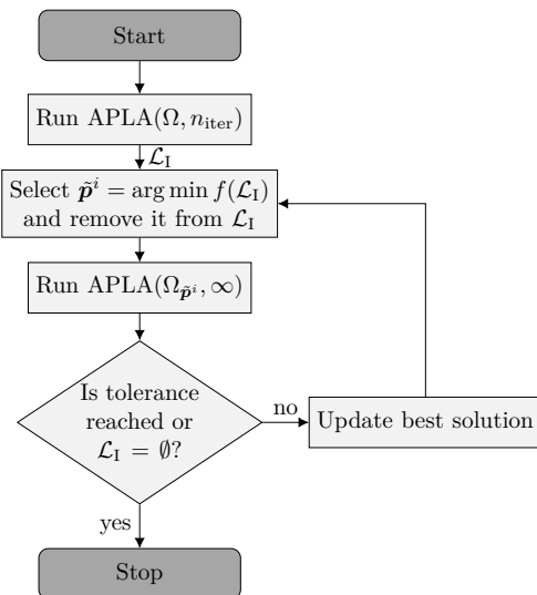
Fig. 3. Flow chart of the APLA-based heuristic.
