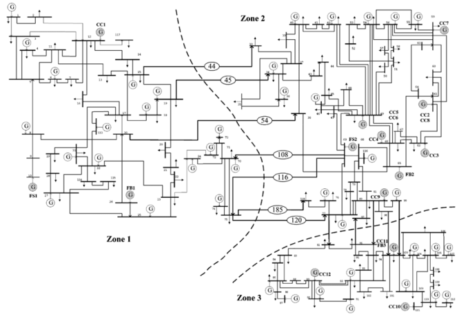
Fig. 7. Single-line diagram of IEEE 118 bus system [17].
